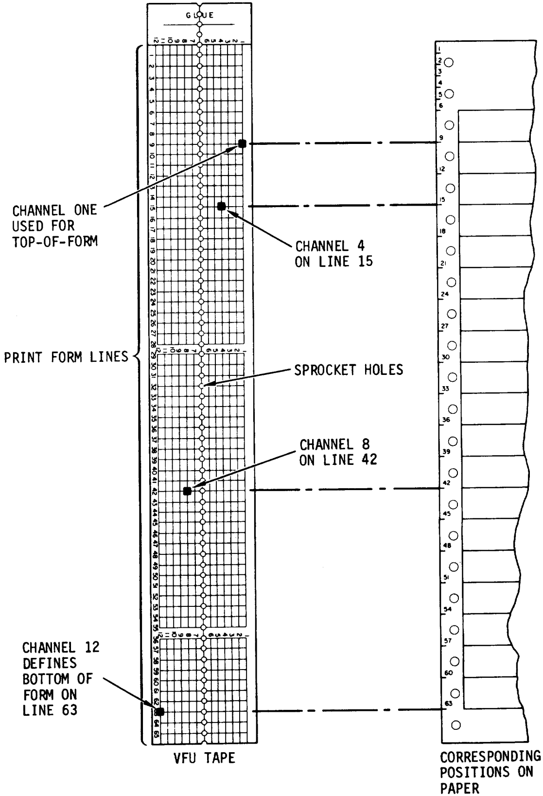
Figure 1-9. Typical VFU Tape Format
